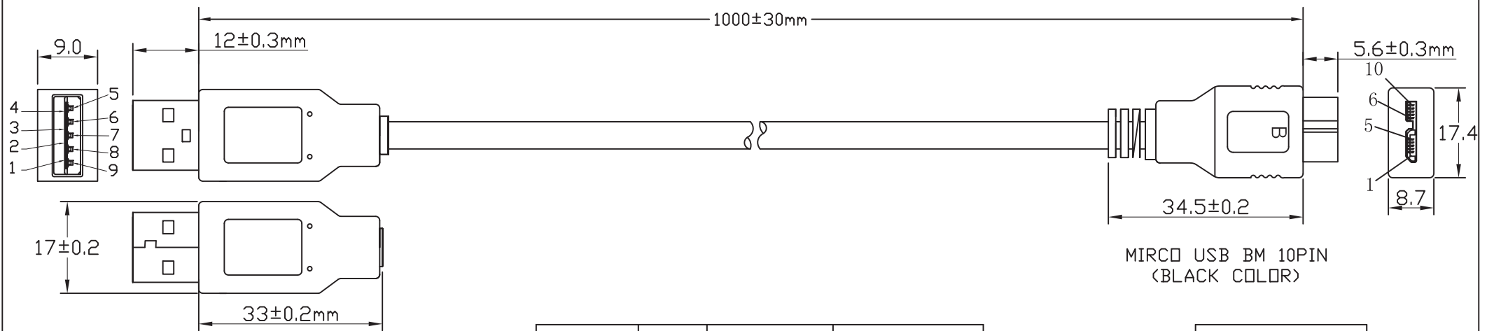
USB3.0 M(A) (BLACK COLOR)
